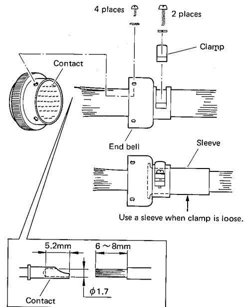
Multi-connector (MQ1602 only)
