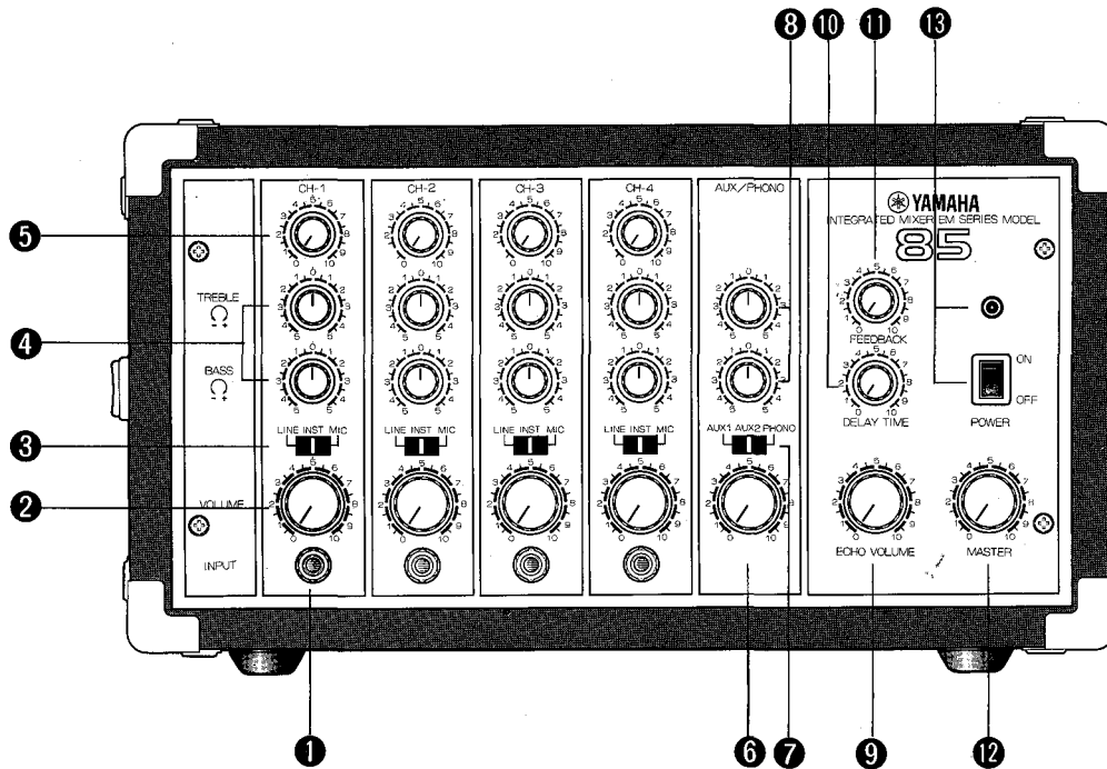
FIG. 1. FRONT PANEL
