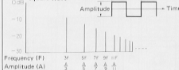
Spectrum of symmetrical square wave
