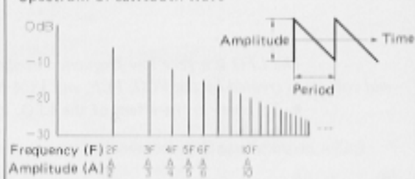
Spectrum of sawtooth wave
