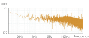
Audio clock jitter of conventional modules
