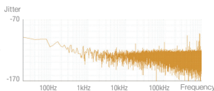
Audio clock jitter of the new module
